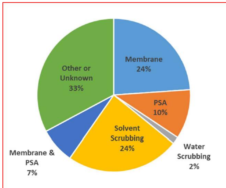
CO2 Removal Technologies for U.S. Manure-Based Biogas-to-RNG Projects in 2018
