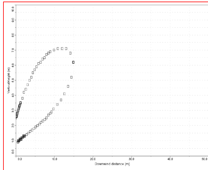
Case 2, 100Pa.g, 1000mm aperture, 30°, D4, half LFL
