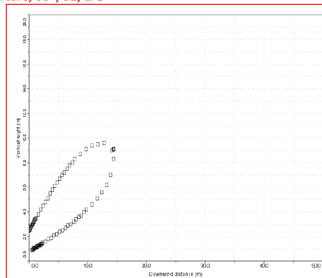
Case 3, 100Pa.g, 1000mm aperture, 30°, B2, LFL
