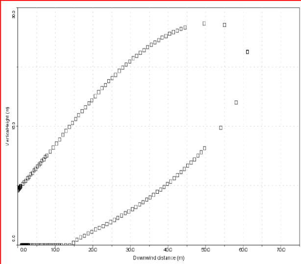
Case 6, 100Pa.g, 5000mm aperture, 15°, D4, LFL
