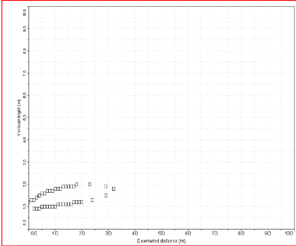
Case 5, 50Pa.g, 200mm aperture, 30°, D4, half LFL
