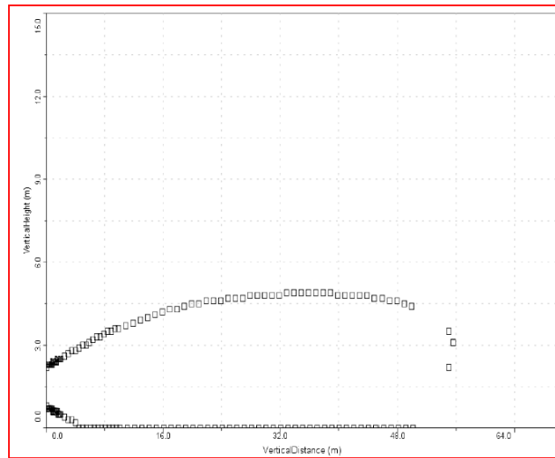
Case 4, 200Pa.g, 1000mm aperture, 0°, D4, half LFL (Rivalea test)
