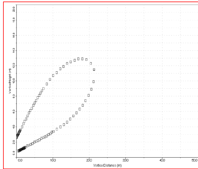
Case 4, 200Pa.g, 1000mm aperture, 15°, D4, LFL (Rivalea test)
