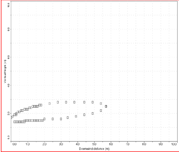
Case 5, 50Pa.g, 200mm aperture, 30°, D4, half LFL
